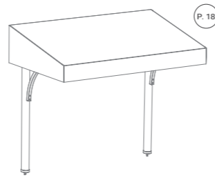
CANOPY L71" W33.5" H61" L180cm W85cm H155cm Fits large units
