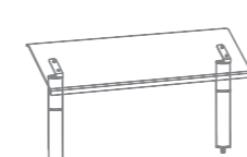
47" HIGH BREATH GUARD H24.5" | gap H14" H62cm | gap H36.5cm Fits medium units
