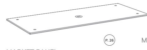
MARKET PANEL (Only for Market Square) L71" W29.5" | L180cm W75cm
