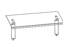
47" BREATH GUARD H18.5" | gap H8.5" H47cm | gap H22cm Fits medium units
