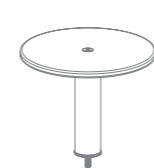
18" ROUND HIGH DISPLAY SHELF Ø18" H12.5" Ø46cm H32cm
