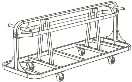
LARGE PLATE TRANSFER AND STORAGE CART L86.5" W31" H36.5" L220cm W79cm H92.5cm holds up to 18 tabletops
